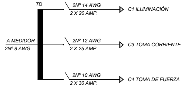
DIAGRAMA UNIFILAR
