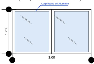
V Ventana (2,00x1,20)
