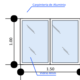
V Ventana (1,50×1,00)
