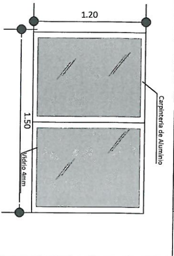
V 1 Ventana (1,50x1,20)
