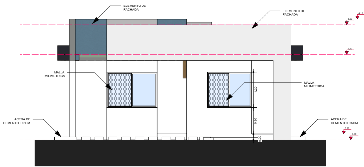
10 FACHADA PRINCIPAL Scale: 1:75
