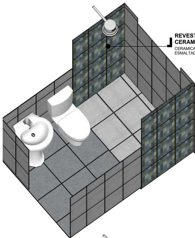
ISOMETRIA
