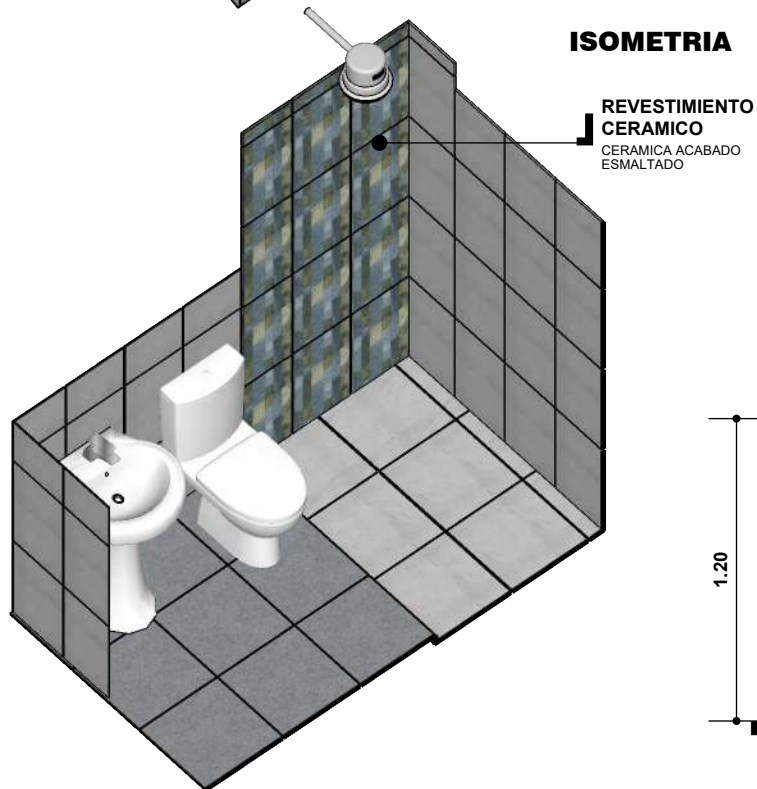
ISOMETRIA
