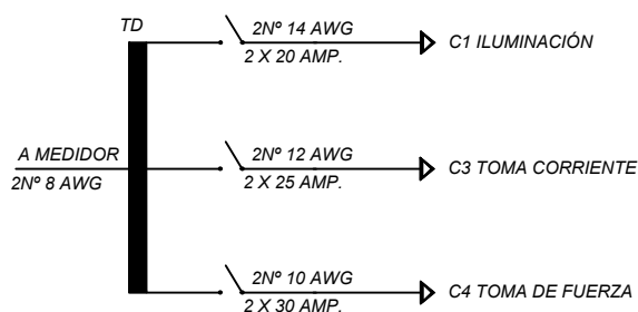
DIAGRAMA UNIFILAR
